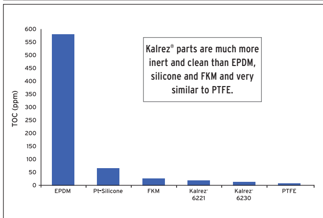
EPA method 415; TOC tests performed on 1" sanitary seals, immersed in 50 mL of sterile WFI at 100°C/24 hrs. The solution was then diluted to 100 mL and analyzed
